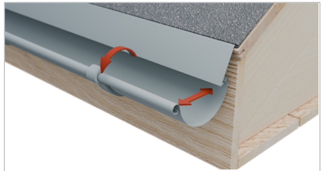
Press the gutter slightly together and twist the gutter down into the bracket lock at the front edge.
